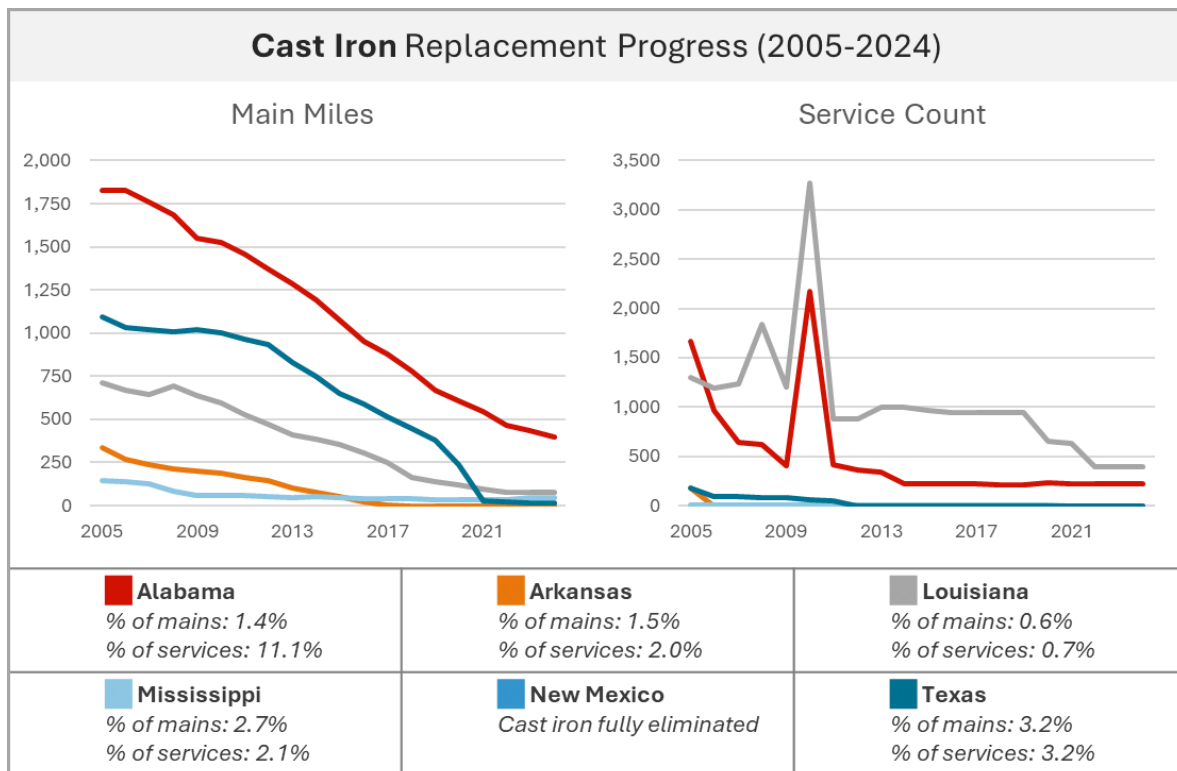
Figure 42. Remaining cast iron pipe in natural gas distribution
