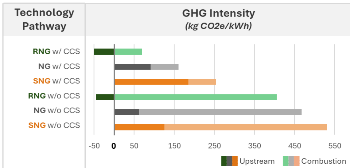
Figure 24. Expected emissions for natural gas power generation in the Gulf Coast
