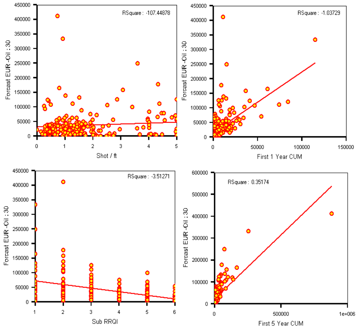
Figure B-5. Regression analysis of four of the parameters versus 30 Year EUR.
