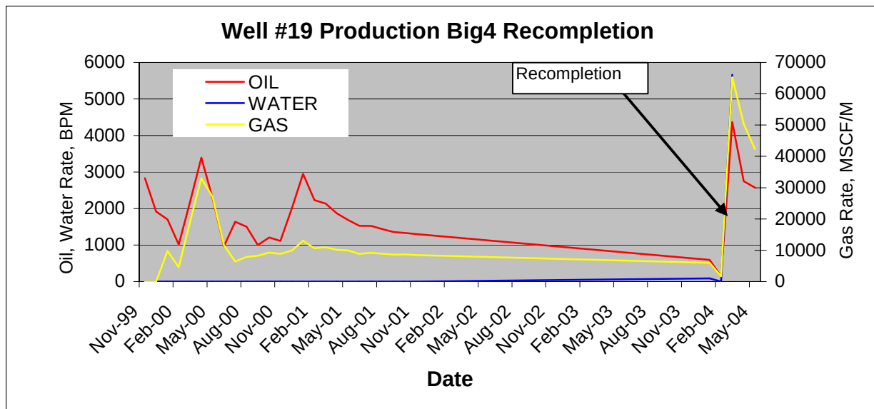
Figure 39: Well #19 monthly production before and after recompletion work
