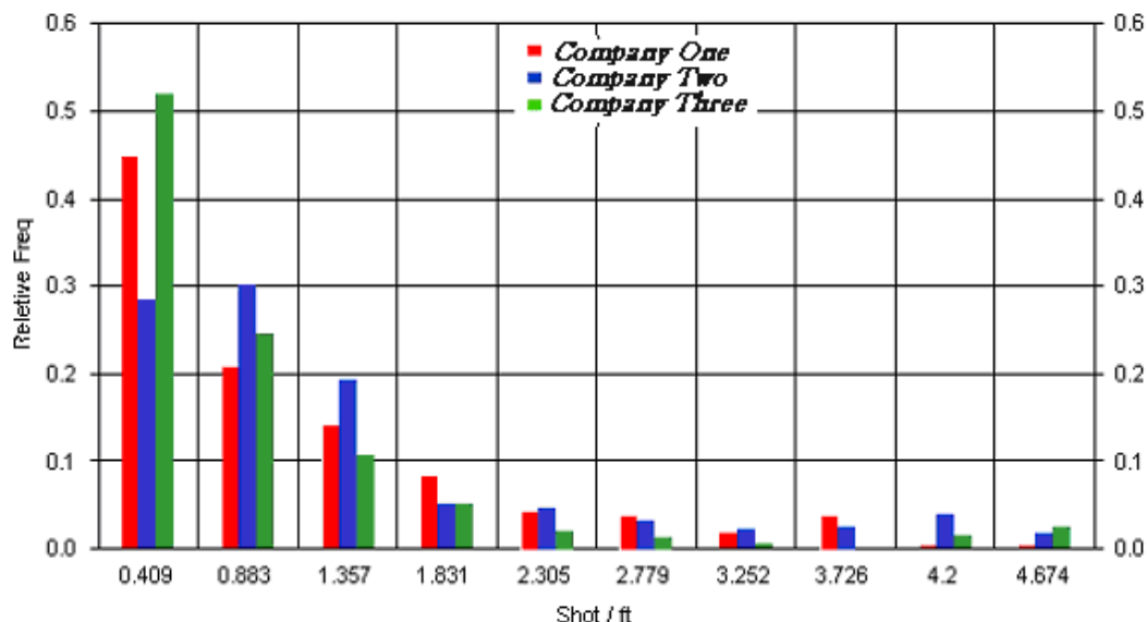
Figure 90: Groups of wells Combinatorial Predictive Best practices Analysis – Results for number of perforations per foot of pay thickness.
