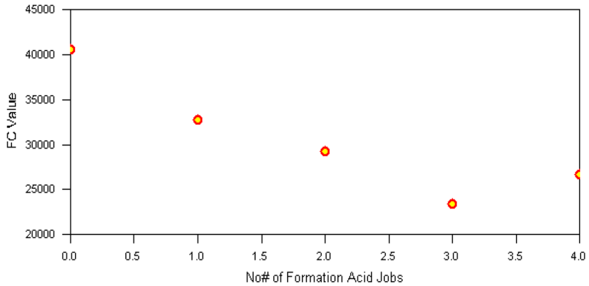
Figure A-25. Influence of Number of formations with Acid Jobs on 30 Year EUR.
