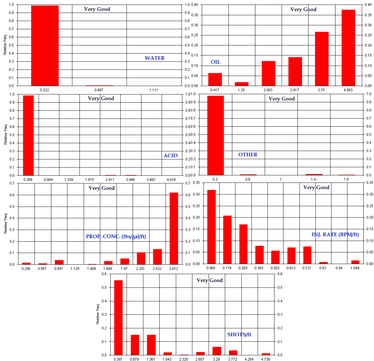
Figure 101: Combinatorial Analysis for Very Good Wells.
