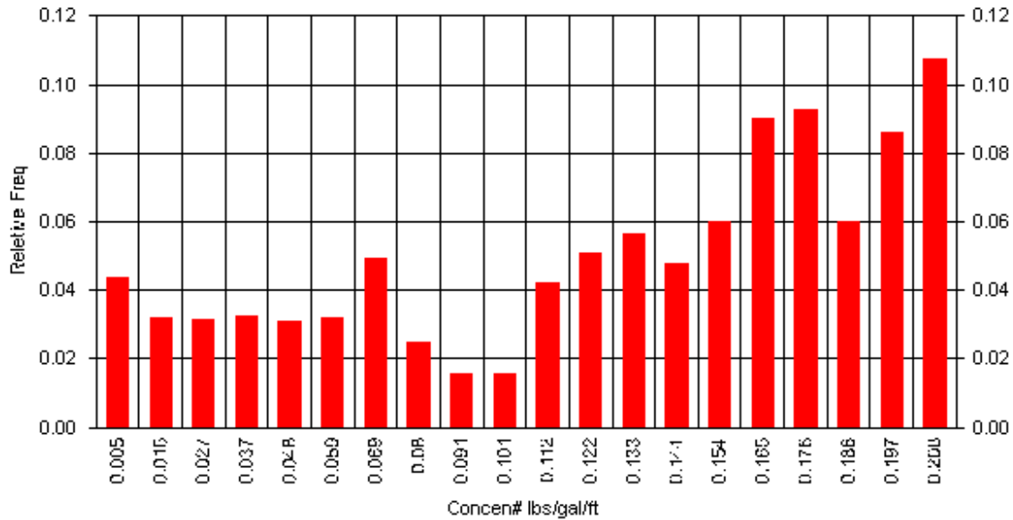
Figure 133: Full field combinatorial analysis for proppant concentration per foot of pay
