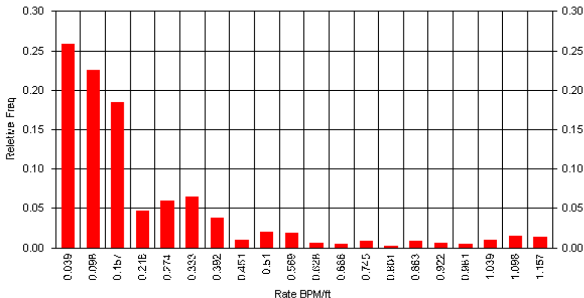
Figure 82: Full Field Combinatorial Predictive Best practices Analysis – Results for the averaged injection rate per foot of Pay Thickness.
