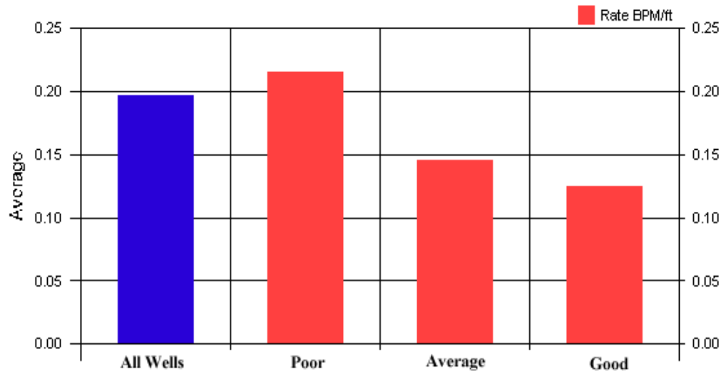
Figure 57: Distribution of the average value of “Average Injection Rate (BPM)/ft” in wells of different quality
