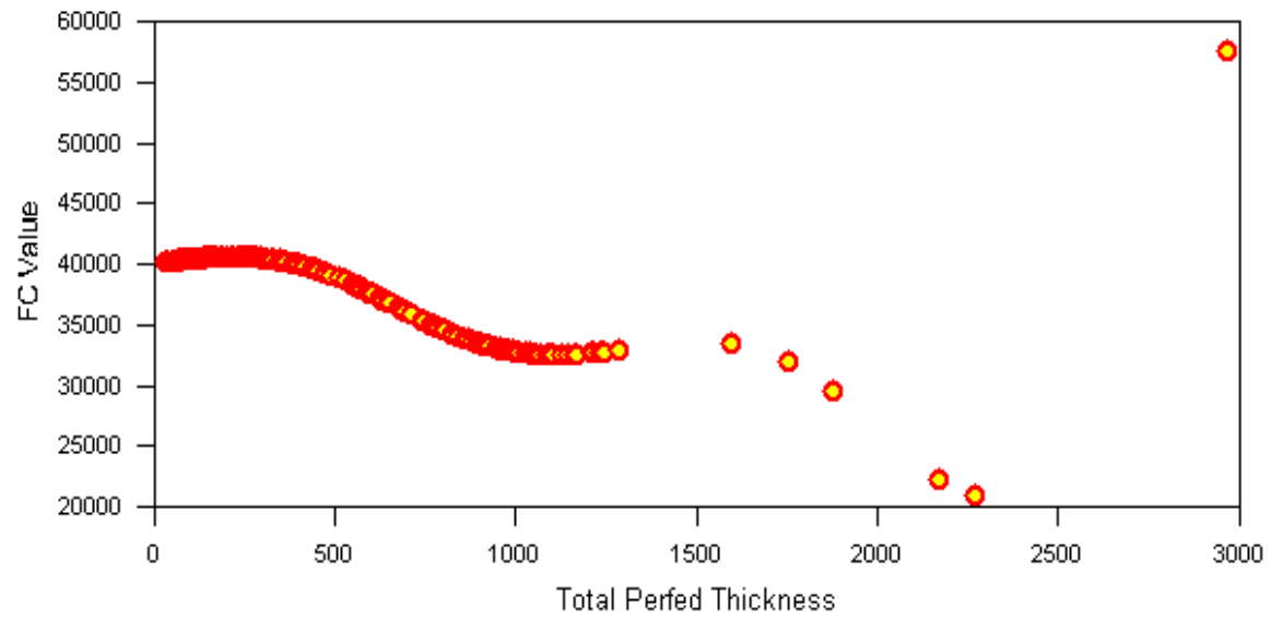
Figure A-1. Influence of Total Perforated Thickness on 30 Year EUR.
