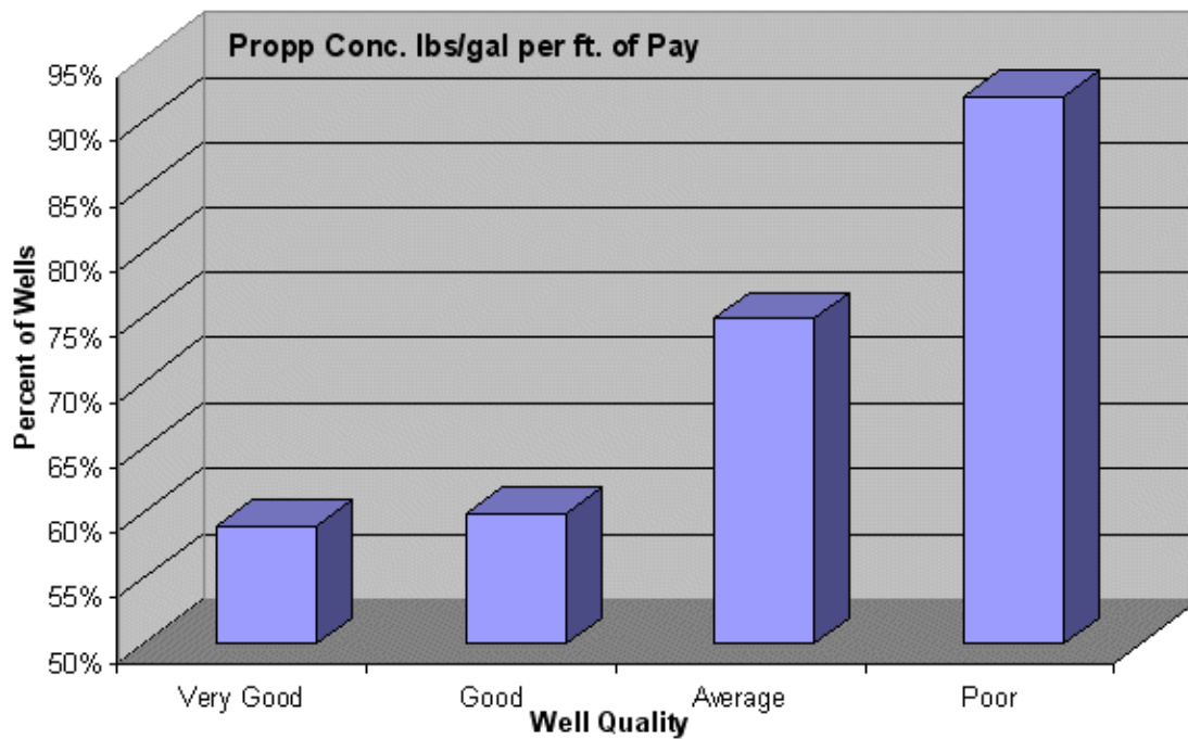
Figure 139: Groups of Wells Analysis for proppant concentration per foot of pay.
