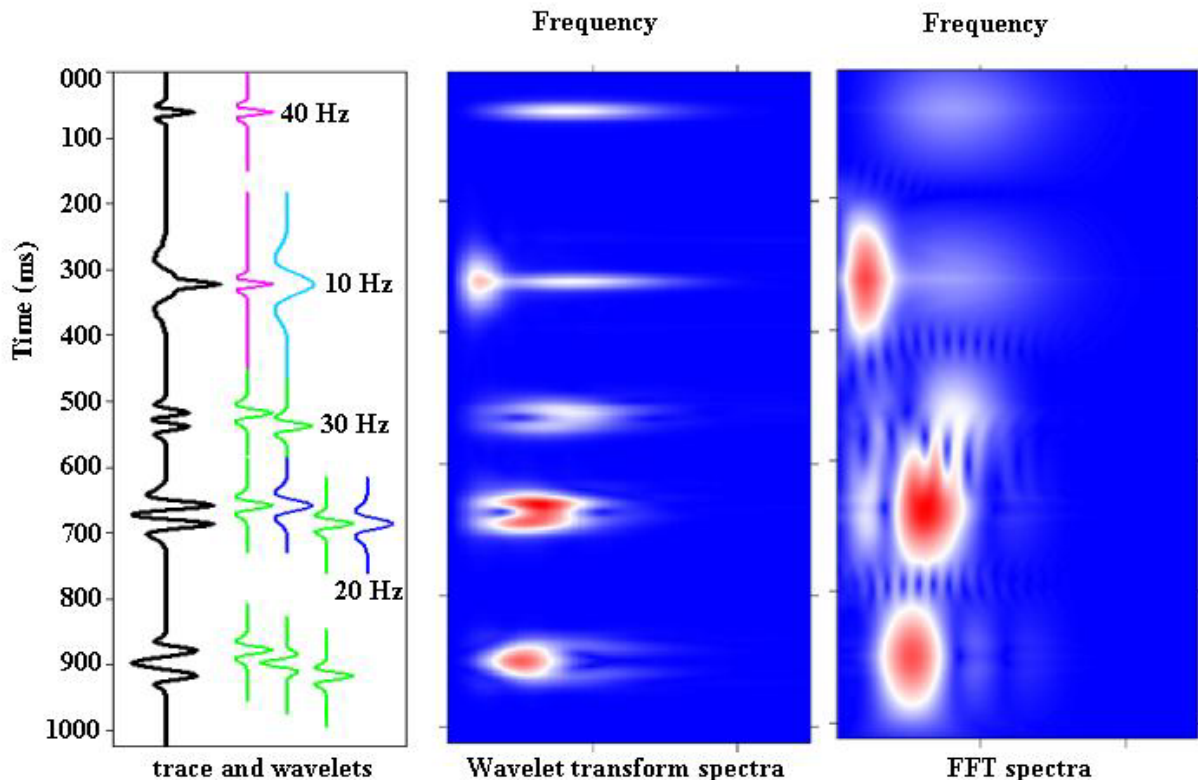
Figure 18: After Castagna et al., 2002. Box at left shows synthetic seismic trace broken down into component wavelets. Boxes at right show comparison between spectra generated by the wavelet transform based method and the Fast Fourier Transform based method. Note windowing problems associated with the Fast Fourier Transform based method, as well as spectral notches, and lack of definition of high frequency components as shown at left.
