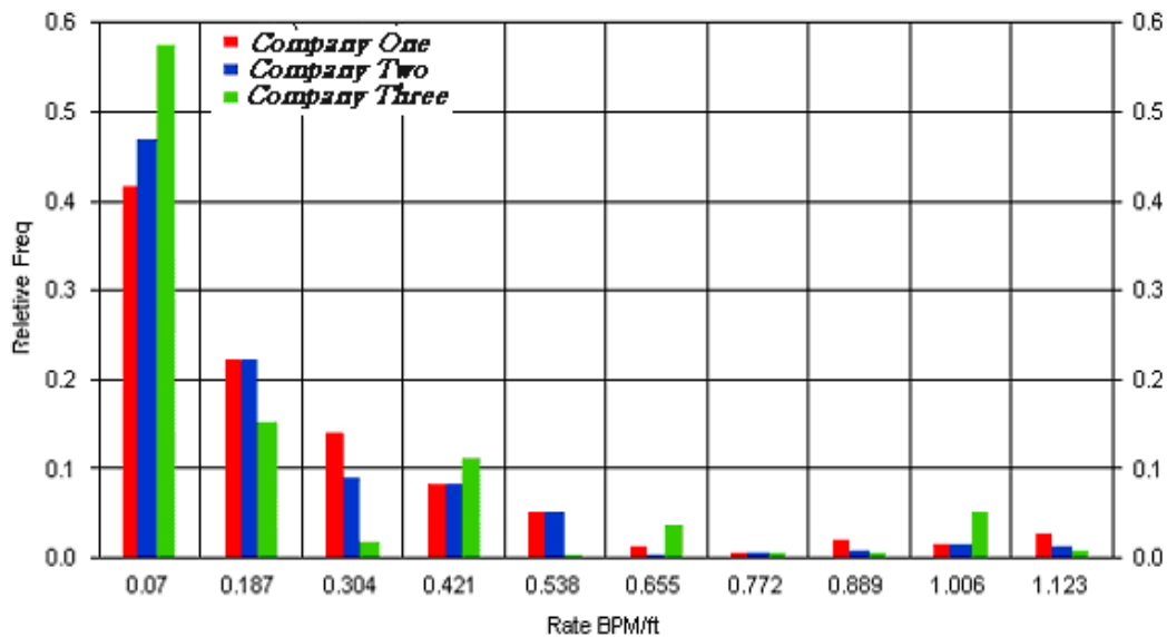
Figure 92: Groups of wells Combinatorial Predictive Best practices Analysis – Results for average injection rate per foot of pay thickness.
