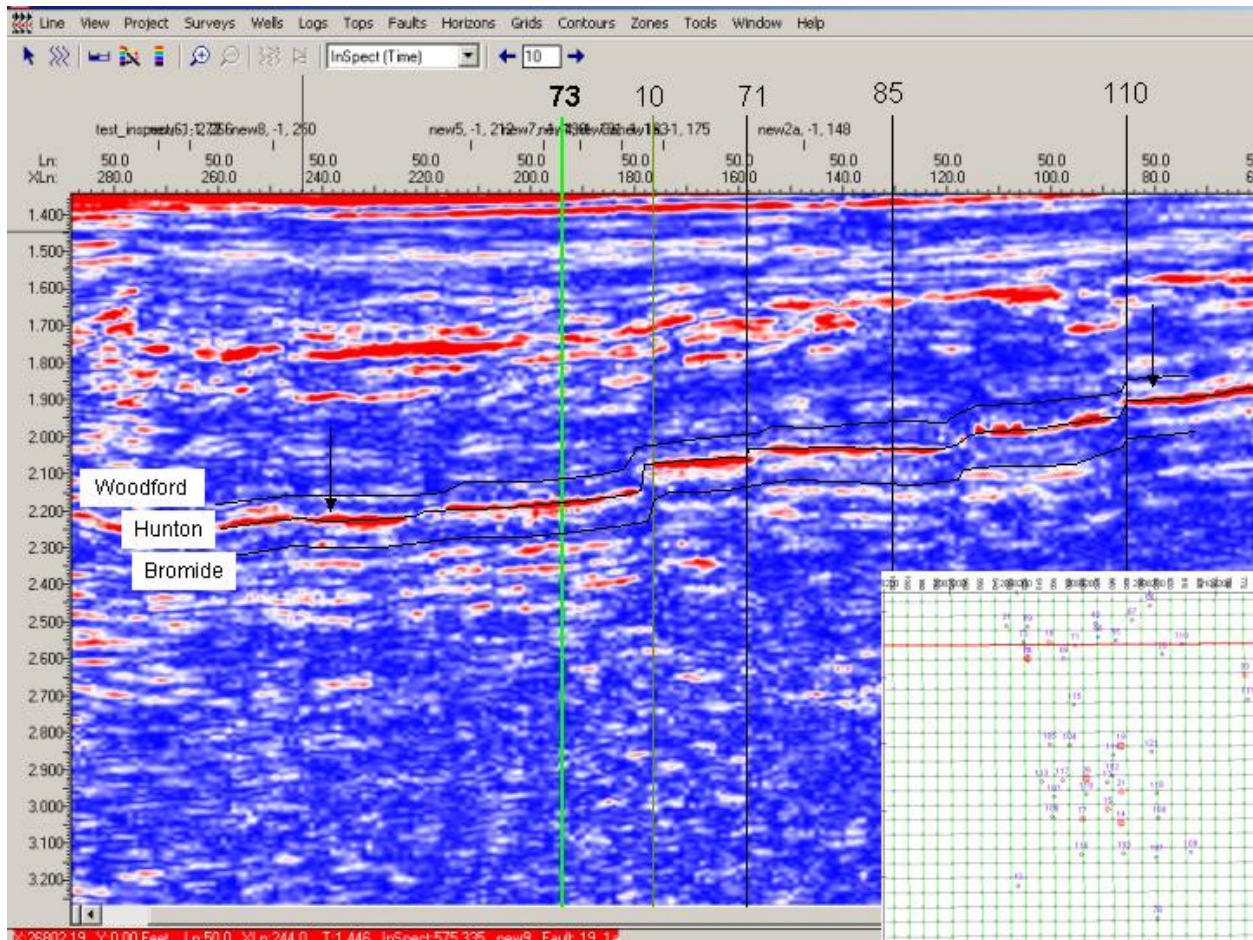
Figure 21: Spectrally decomposed data at 50 Hz along line through good producer 73 (bright green vertical line) and proposed location 110. Inset shows line in map view. Vertical dimension is two-way travel time. Red represents high energy (amplitude) at this frequency, white intermediate, and blue low. The Woodford, Hunton, and Bromide horizons are highlighted for interpretation
