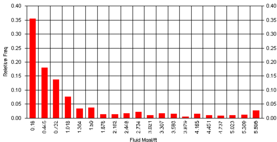
Figure 132: Full field combinatorial analysis for amount of fluid pumped per foot of pay
