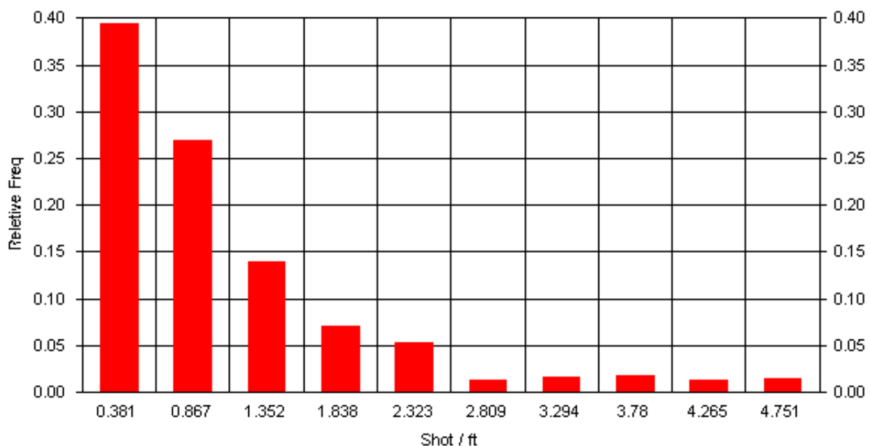
Figure 80: Full Field Combinatorial Predictive Best practices Analysis – Results for number of perforations per foot of Pay Thickness.
