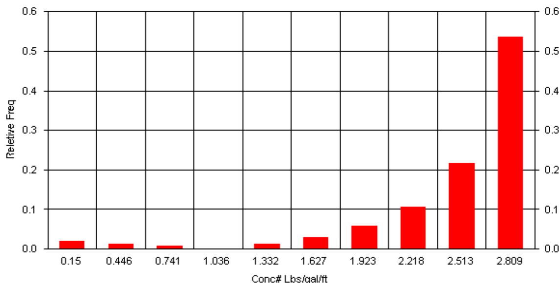
Figure 81: Full Field Combinatorial Predictive Best practices Analysis. Results for proppant concentration in pounds per gallon of fluid per foot of pay thickness.
