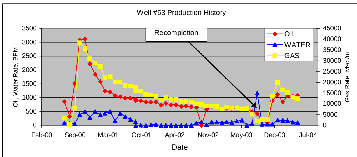
Figure 40: Well #53 monthly production before and after recompletion work
