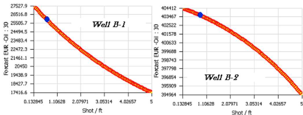
Figure 103: Sensitivity analysis for number of perforations per foot of pay thickness for two wells in the database.
