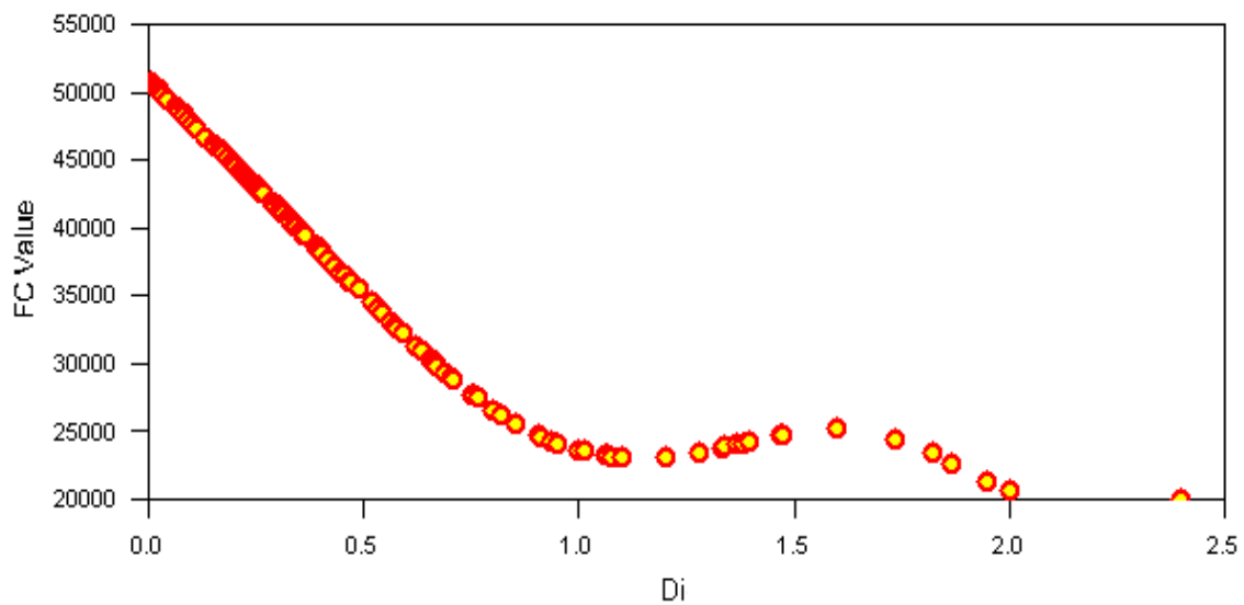
Figure A-18. Influence of Decline Curve Analysis Initial Decline Rate on 30 Year EUR.
