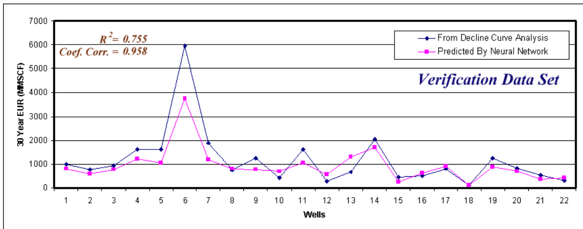
Figure 127: Decline curve versus network predicted gas 30 year EUR for the verification set
