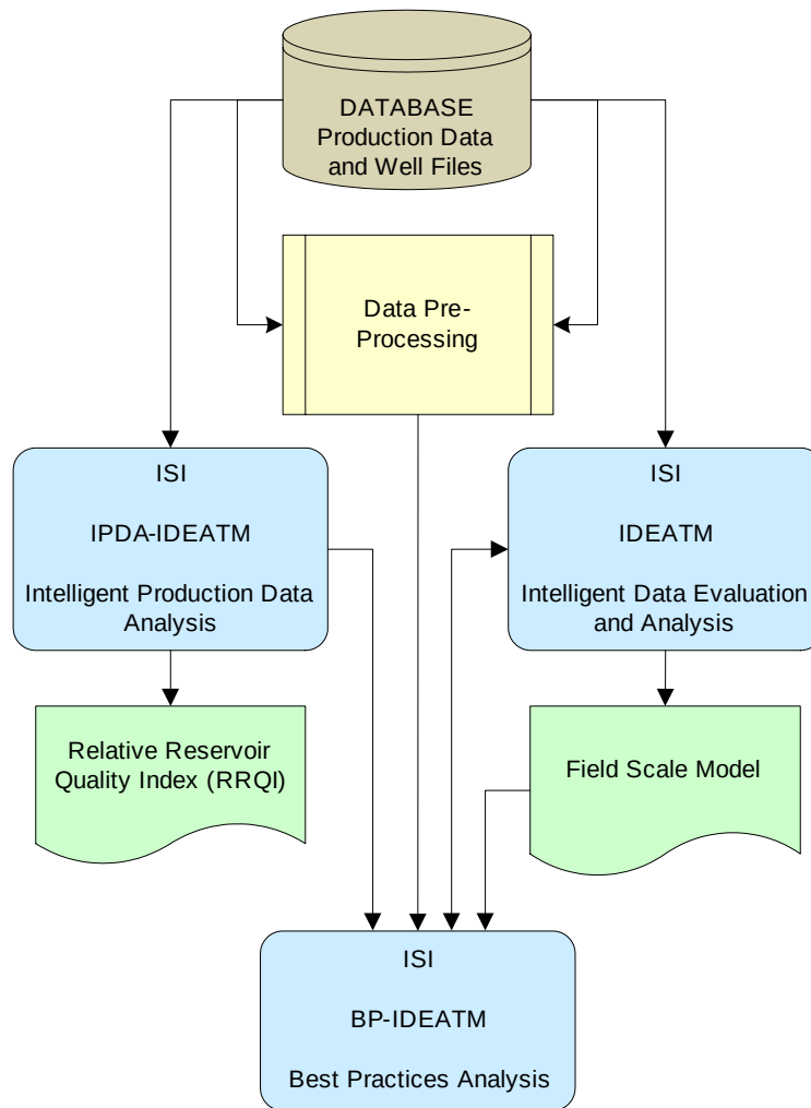
Figure 62: Flow chart of Best Practices Analysis using Artificial Intelligence Techniques.
