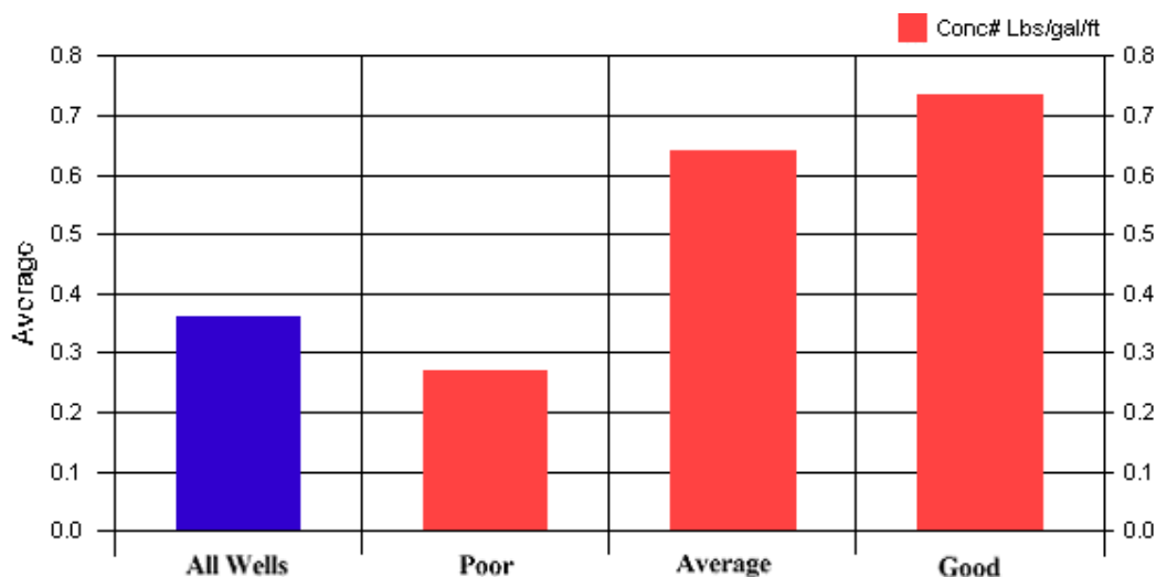
Figure 56: Distribution of the average value of “Average Proppant Concentration (lbs/gal/ft) in wells of different quality
