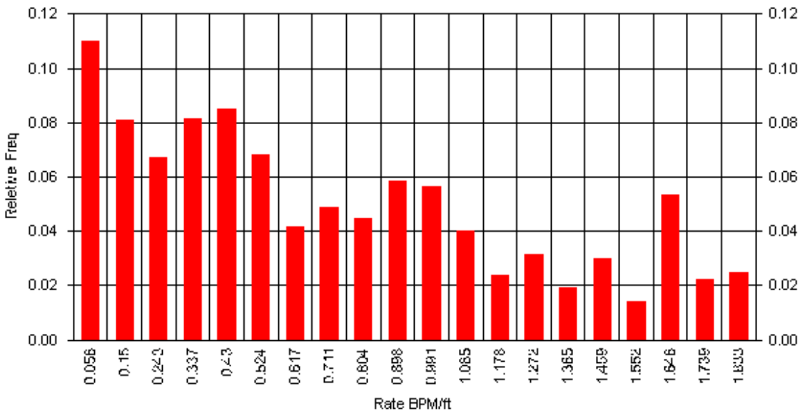
Figure 134: Full field combinatorial analysis for average injection rate per foot of pay
