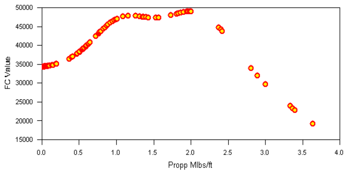
Figure A-6. Influence of Proppant Amount of pay on 30 Year EUR.
