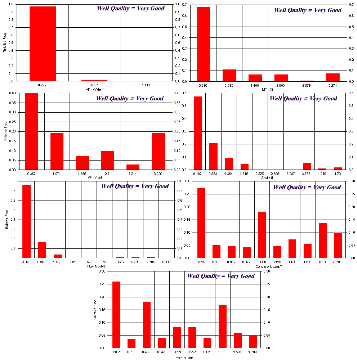
Figure 141: Groups of Wells Analysis combinatorial analysis for very good wells.
