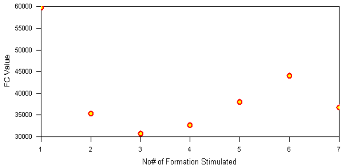
Figure A-23. Influence of Number of formations Stimulated on 30 Year EUR.
