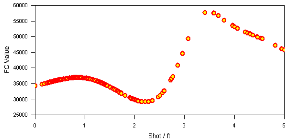
Figure A-2. Influence of Total Shots per foot of pay on 30 Year EUR.
