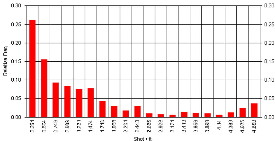
Figure 131: Full field combinatorial analysis for number of perforations per foot of pay.
