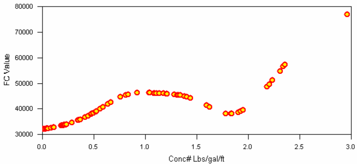
Figure A-26. Influence of Proppant Concentration on 30 Year EUR.
