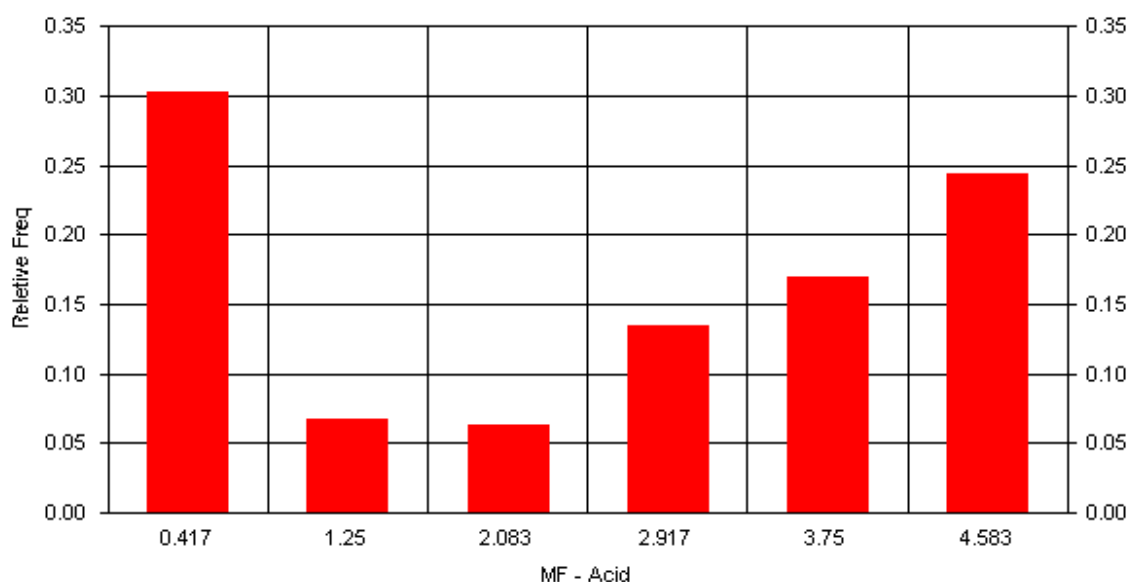
Figure 130: Full field combinatorial analysis for acid as the main stimulation fluid.
