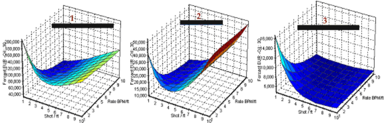
Figure 104: Sensitivity analysis for “Shot/ft” and “Rate” for three wells in the database.
